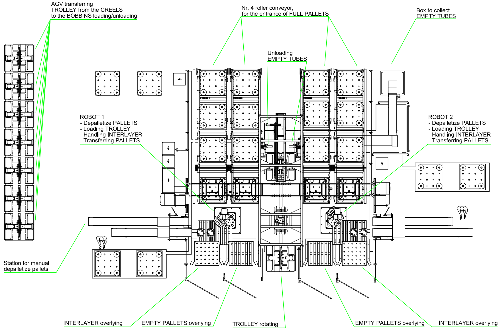
AUTOMATIC CREELING SYSTEM for TUFTING MACHINES (ARTIFICIAL GRASS)
