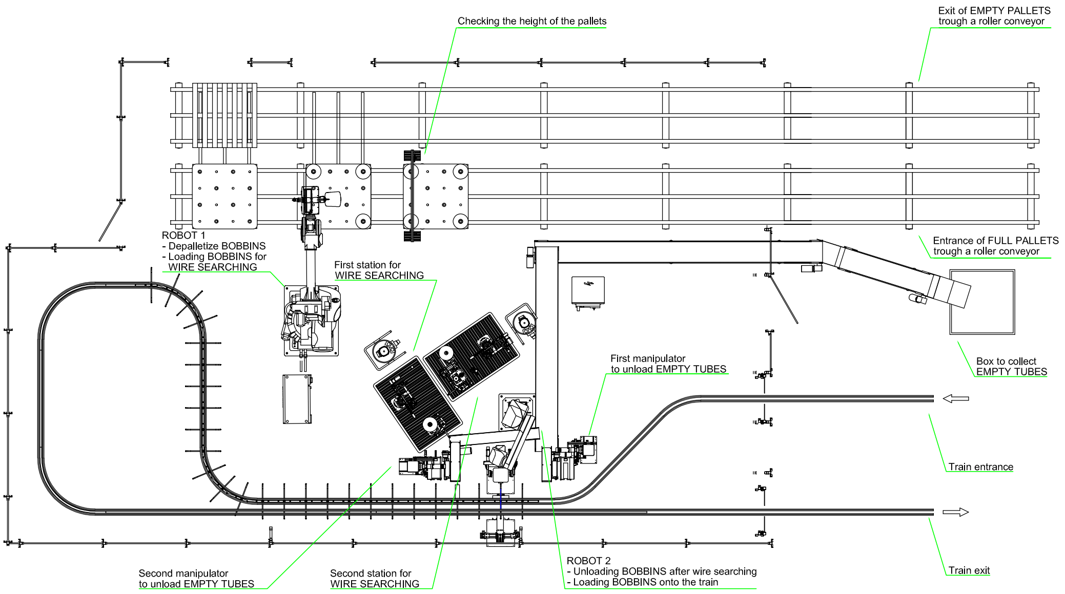
AUTOMATIC CREELING SYSTEM for TUFTING MACHINES (CARPET)
